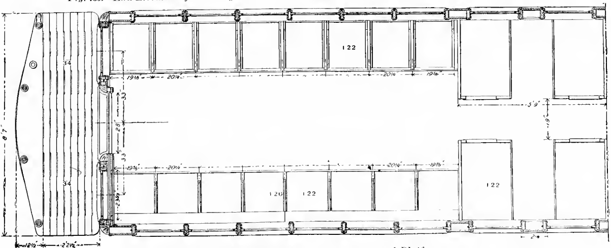
Fig. 467. Sectional Half Plan, Showing Seats and Platform.
